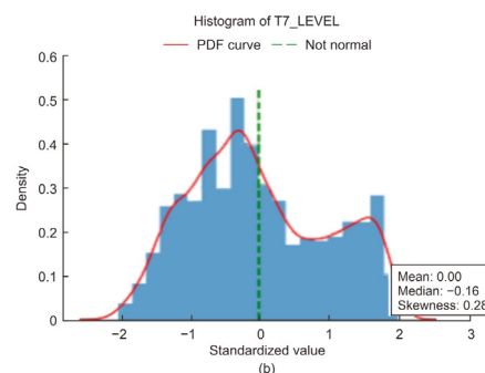
Fig. 14. Normalization and skewness test of features (a) L_T7 and (b) T7_LEVEL.
