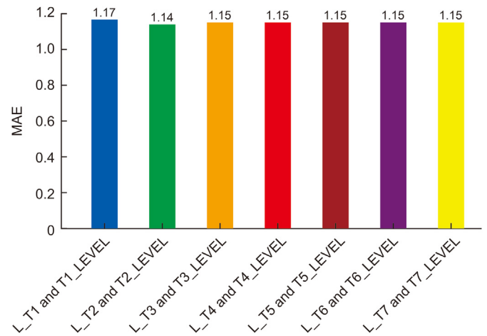
Fig. 15. Mean absolute error (MAE) for each variable pair.
