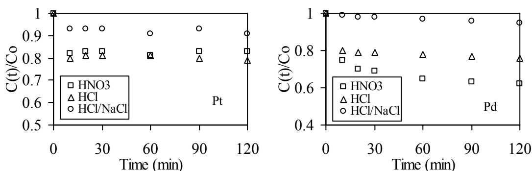
Fig. 5. Influence of the acid used for pH control on Pt and Pd sorption kinetics at pH 2 using D. desulfuricans ( C_0(\text{Pt/Pd}) : 50 mg Metal \text{L}^{-1} ; Sorbent dosage: 150 mg \text{L}^{-1} ).
