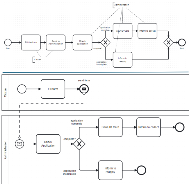
Figure 6. Process model from the FPD (upper model) vs. expected process model (lower model)
