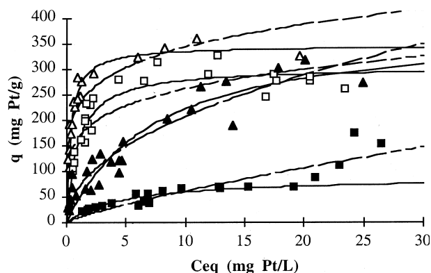
Figure 7. Influence of the acid used for pH control (open symbols, HCl; closed symbols, H 2 SO 4 ) at pH 2 on platinum sorption isotherms using either TGC-3:2:1 (△) or GCC-2:1 (□). Solid lines: Langmuir modeling; dashed lines: Freundlich modeling.
