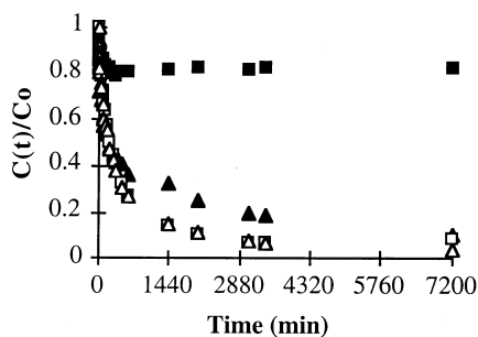
Figure 10. Platinum sorption kinetics at pH 2 using TGC-3:2:1 ( \Delta/\blacktriangle ) and GC-2:1 ( \square/\blacksquare ) ( C_0 : 10 \text{ mg L}^{-1} , sorbent dosage: 50 \text{ mg L}^{-1} , for HCl-controlled pH solution (open symbols); sorbent dosage: 100 \text{ mg L}^{-1} for \text{H}_2\text{SO}_4 -controlled pH solutions (closed symbols)).
