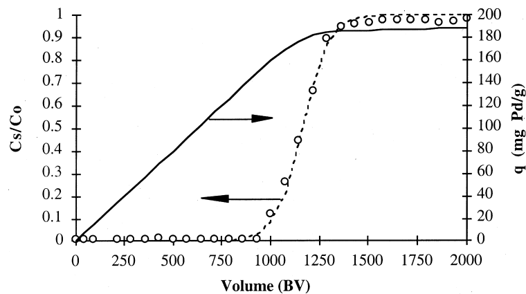
Figure 13. Breakthrough curve for palladium sorption on GCC-2:1 at pH 2.
