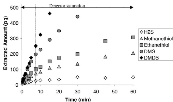
Fig. 2. Variation of time (min) vs. amount extracted for a mixture of sulphur compounds: about 10 \mu\text{g m}^{-3} for each component (desorption temperature, 250 \text{ }^\circ\text{C} ; desorption time, 2 min).
