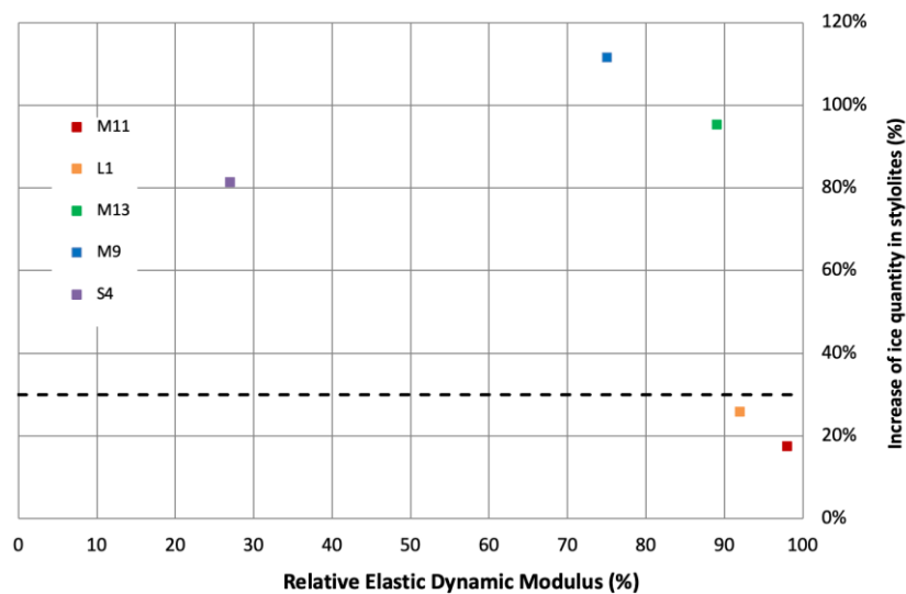
Fig. 18 Relation between increase of ice quantity inside stylolite and RDEM
