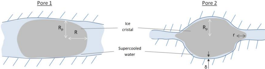
Fig. 4 Two pores shapes with different entry radii : pore 1 with large entry radius and pore 2 with small entry radius. Stresses induced during freezing are higher in pore 2 than pore 1 because of the high interface curvature ( R \gg r ) [17, 18]
