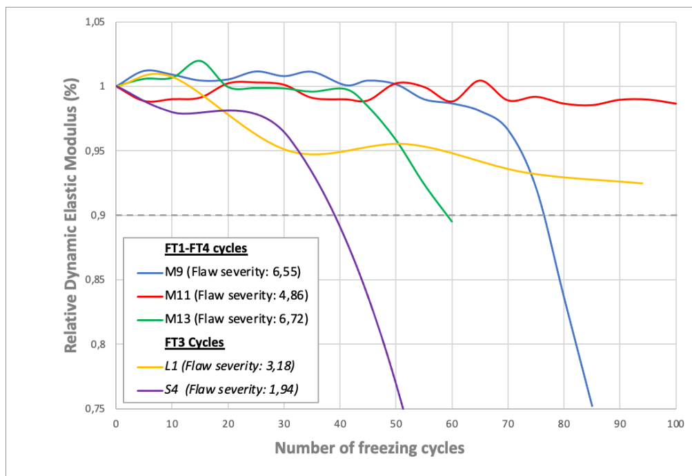
Fig. 14 Evolution of Relative Dynamics Modulus of Elasticity as a function of the number of FT cycles
