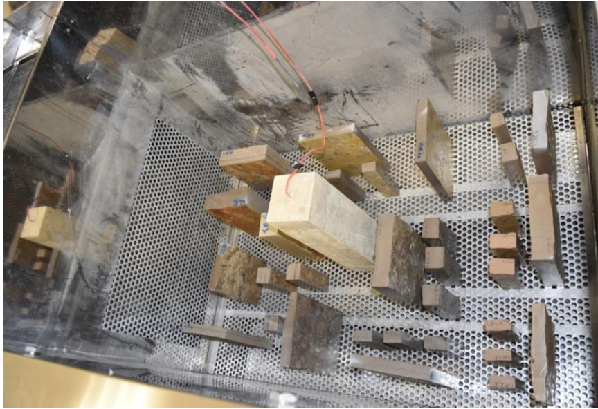
Fig. 13 Samples in the freeze/thaw chamber model CHD – 525
