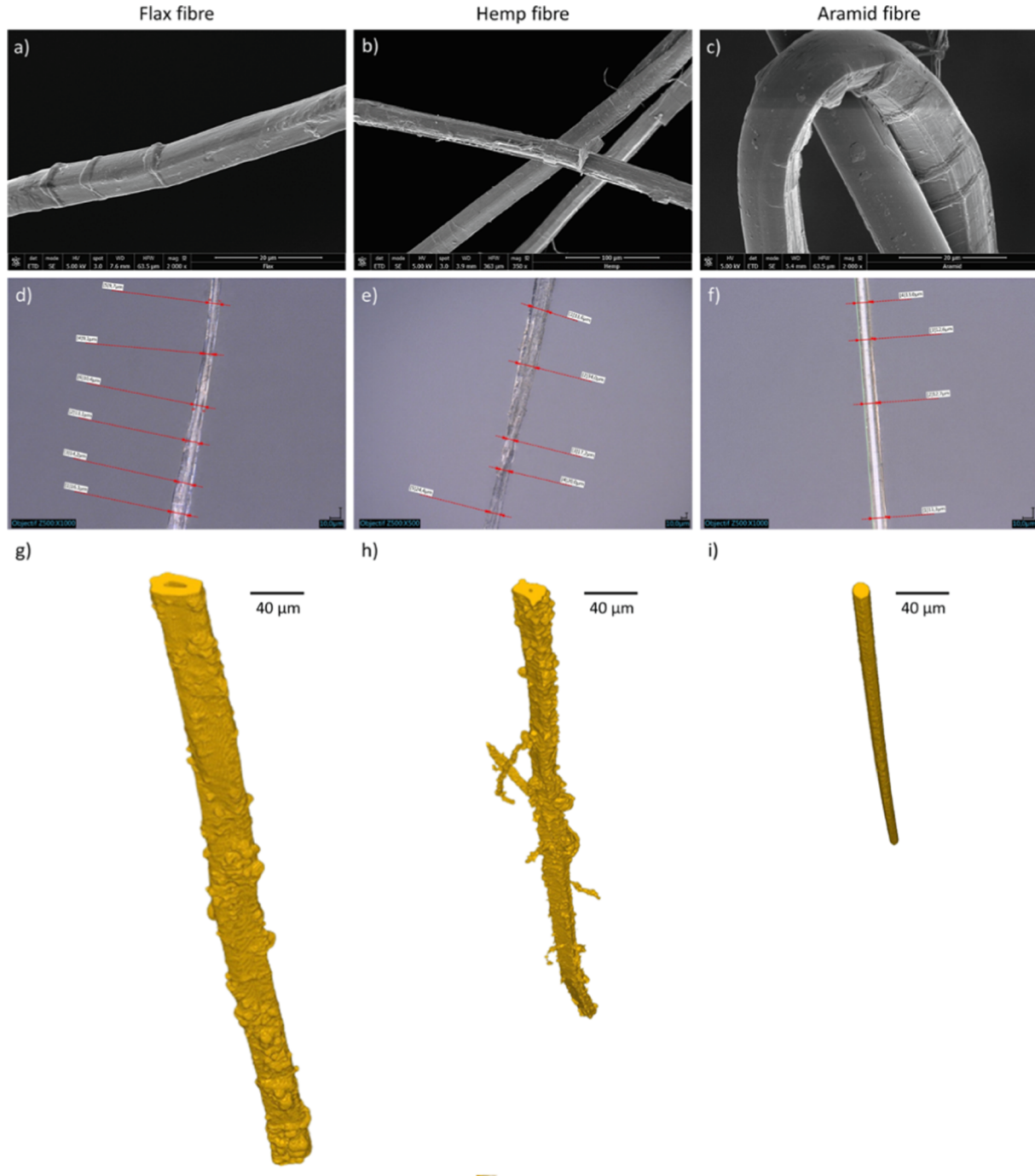
Fig. 1. (a-c) SEM and (d-f) light optical micrographs of flax, hemp and aramid fibres. (g-i) 3D-rendered perspective views (voxel size: 0.35^3 \mu\text{m}^3 ) of the three types of fibres obtained using synchrotron X-ray microtomography (BM05 beamline, ESRF, Grenoble, France).
