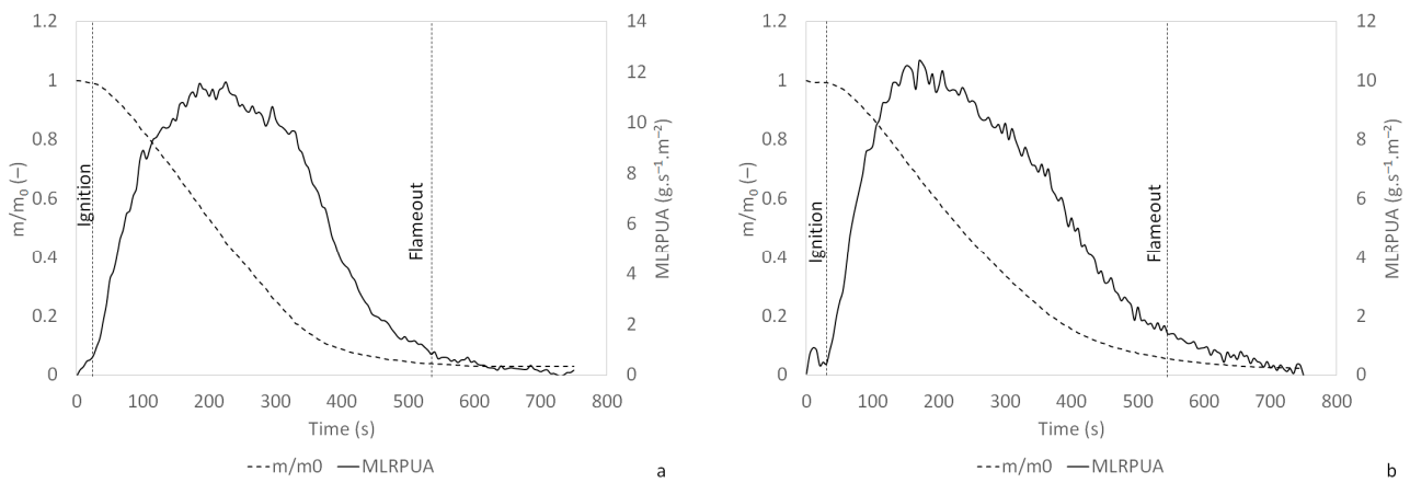
Figure 10. Mean mass and MLRPUA for (a) PPr r composite and (b) HDPE r composite—with a cork content of 15 wt%.
