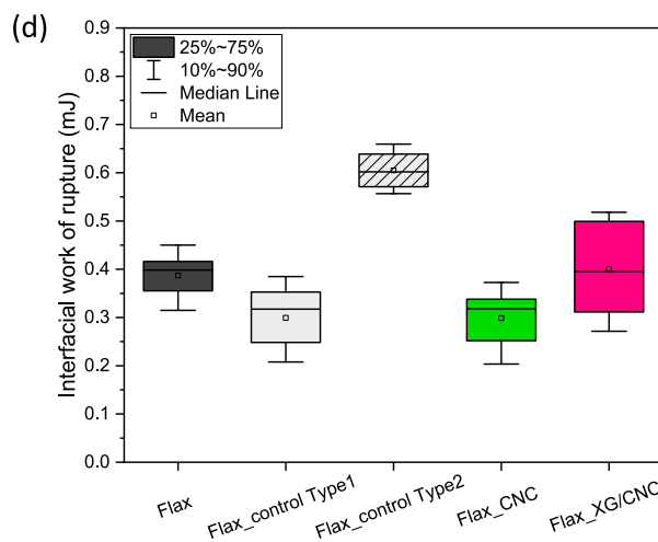
Fig. 3. (a) box charts of the IFSS measured by microbond tests with epoxy droplets on raw flax, flax_control , flax_CNC and flax_XG/CNC elementary fibres with (b) related mean and median values; (c) force–displacement curves with the two types of debonding behaviour observed with microbond tests; (d) box charts of the interfacial work of rupture.
