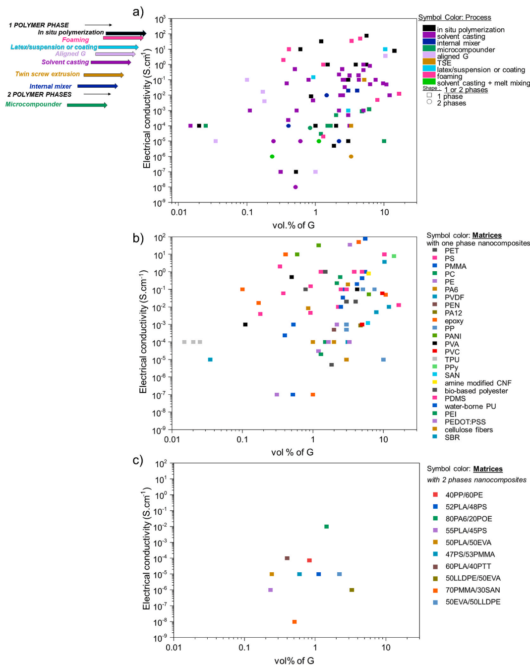
Fig. 29. Graphs representing the electrical conductivity versus vol% of graphene based on references [3,7,59,60,62,66,78,84,111,126,136,137,143,148,150,152,166,167,169,172]– [178,180–226]. (a) Effect of process and the number of polymer phases (one or two phases), (b) effect of the polymer matrices for one phase nanocomposites, (c) effect of the polymer matrices for two phases nanocomposites, (d) effect of the type of graphene or graphite used and (e) effect of the nanoparticle localization into the blend among the references dealing with polymer blends. (A colour version of this figure can be viewed online.)
