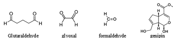
FIGURE 1 Main crosslinking agents of casein-based compounds.
