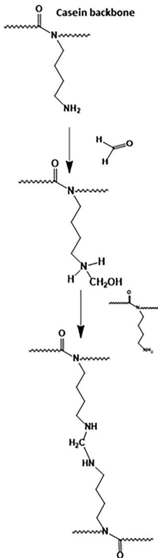
FIGURE 3 Reaction scheme of casein crosslinking with formaldehyde.
