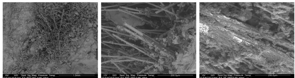
Figure 10. SEM observations of the fractured surface of the cement mortar containing 10% GFRP (BSE).
