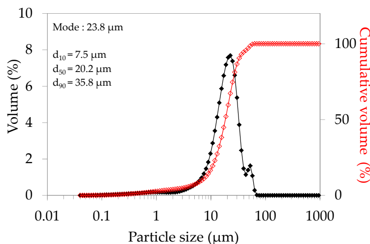
Figure 2. Particle size distribution of the cement.
