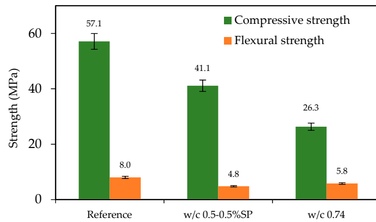
Figure 8. Compressive strength of the cement mortar with 15% GFRP.
