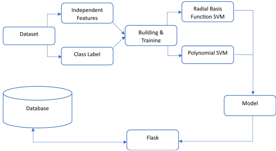
Fig. 3. Model architecture.
