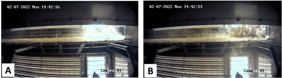
Figure 9. Ignition stage of the cable layer (seen from camera 1). (A) Increase of IHF imposed on the ignition zone. (B) Ignited cable layer in the ignition zone.
