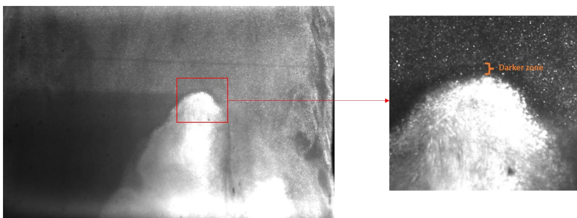
Figure 6: Example of images obtained by PIV (Particle Image Velocimetry)
