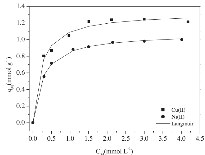
Fig. 2. Sorption isotherms for Cu(II) and Ni(II) recovery from mono-component solutions using acidified Sargassum filipendula (derived from breakthrough curves).
