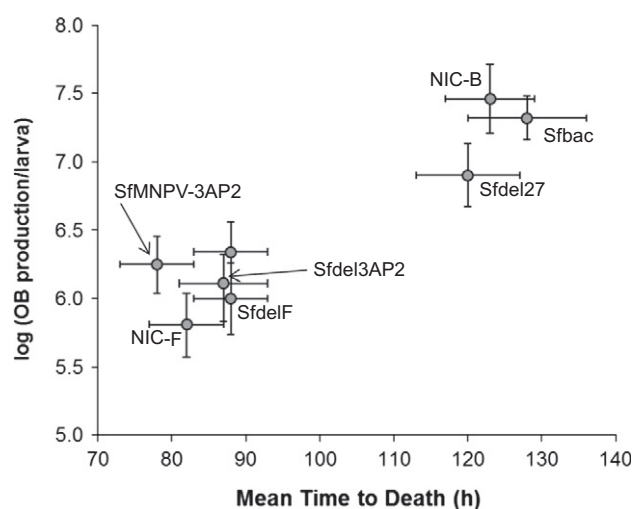
Fig. 1. Mean time to death (h) and log[OB production/larva] characteristics of OBs of NIC-B (SfB), NIC bacmid (Sfbac), NIC-F (SfF), SfdelF bacmid (SfdelF), SfMNPV-3AP2 (Sf3AP2), Sfdel3AP2 bacmid (Sfdel3AP2), Sfdelegt bacmid (Sfdelegt) and Sfdel27 bacmid (Sfdel27) in Spodoptera frugiperda inoculated in the second instar. Horizontal and vertical bars indicate SE of each variable.
