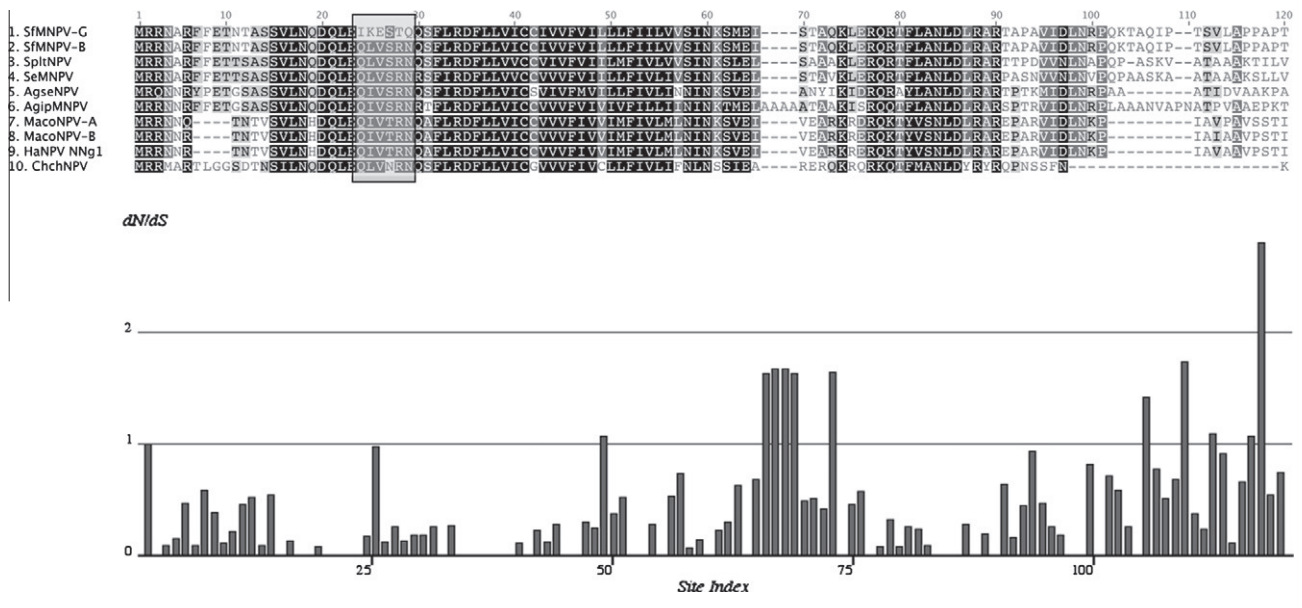
Fig. 1. Multiple sequence alignment of amino acid sequences of SF58 proteins of selected baculoviruses. Gray box indicates the conserved region of SF58 proteins, except in SfMNPV-G. Similarity between amino acids in the same position is indicated by shading (black 100% similar, dark gray 80–100% similar, light gray 60–80% similar and white less than 60% similar). Bar chart represents significant negative selective forces acting on the protein ( P < 0.05 ), positively selected sites ( d_N/d_S > 1 ) were not significant ( P > 0.05 ). Baculovirus sequences used in the comparative analysis were GenBank (accession number); SfMNPV-G (JF899325), SfMNPV-B (HM595733), S. litura NPV (AF325155), S. exigua MNPV (AF169823), Agrotis segetum NPV (DQ123841), A. ipsilon MNPV (EU839994), Helicoverpa armigera NPV Nng1 (AP010907), Mamestra configurata NPV A (U59461), M. configurata NPV B (AY126275) and Chrysodeixis chalcites NPV (AY864330).
