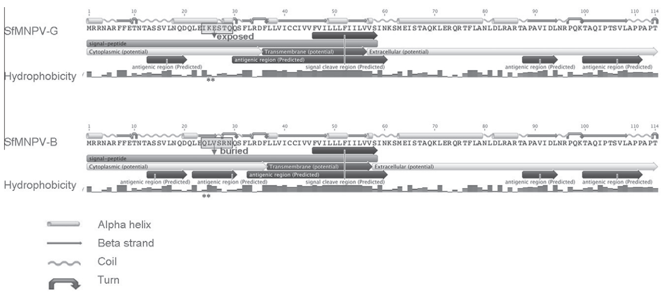
Fig. 2. Amino acid translation of the sf58 gene from (A) SfMNPV-G and (B) SfMNPV-B genotypes. Boxes indicate major changes into the amino acid sequence and secondary structure of the proteins. Asterisks indicate changes into the hydrophobicity of the amino acids. The predicted exposed status of each site, buried or exposed, is indicated.
