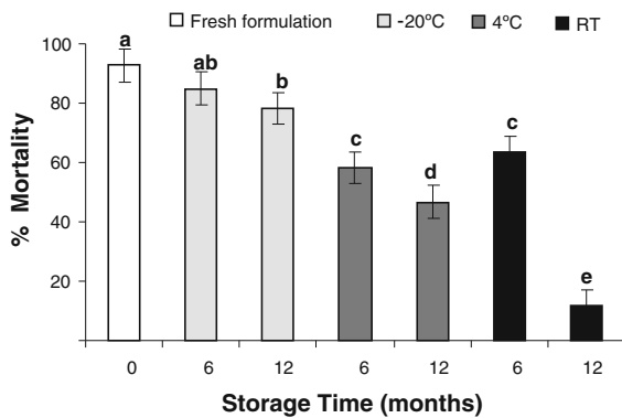
Fig. 2 Mean percentage mortality of T. solanivora larvae treated with liquid formulation samples taken after six and 12 months storage at -20 , 4 °C and ambient temperatures (RT). Columns headed by different letters are significantly different (Tukey test, P < 0.05 ). Bars indicate SE
