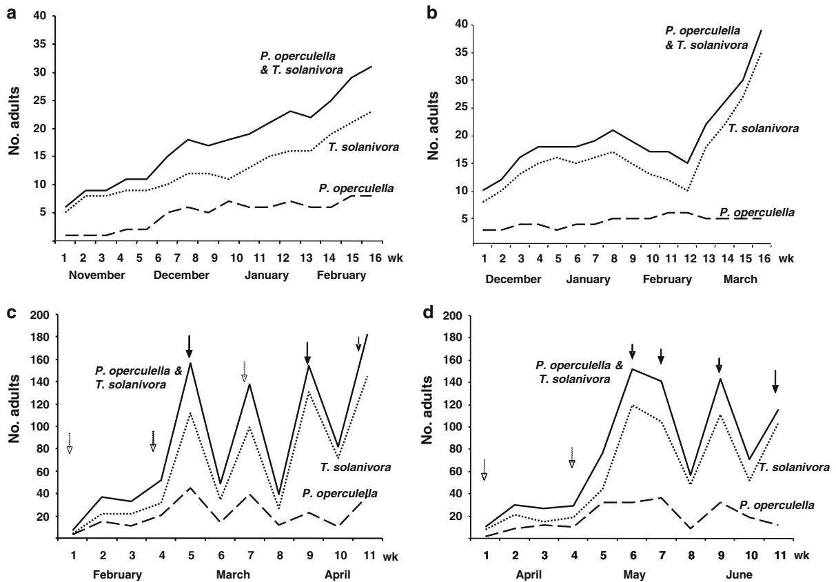
Fig. 1 Changes in the number of male moths of T. solanivora (dotted line), P. operculella (dashed line) or both (solid line) captured in pheromone traps in warehouses ( a , b ) and in potato fields during the dry ( c ) and humid ( d ) seasons. Arrows indicate
