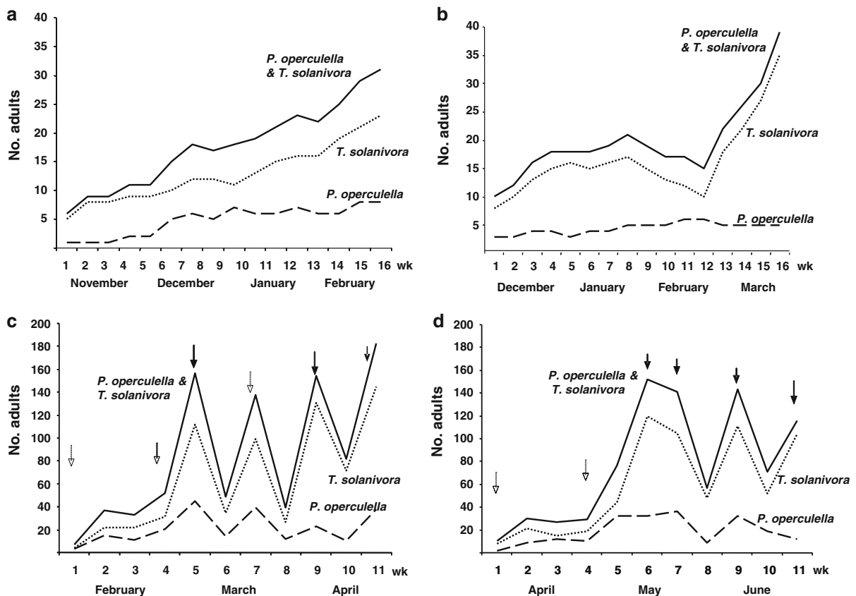
Fig. 1 Changes in the number of male moths of T. solanivora (dotted line), P. operculella (dashed line) or both (solid line) captured in pheromone traps in warehouses (a, b) and in potato fields during the dry (c) and humid (d) seasons. Arrows indicate
