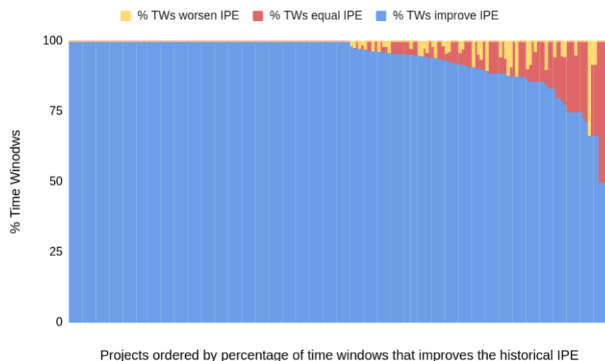
Fig. 9. Percentage of time windows that improves, maintains and worse the historical IPE by project
