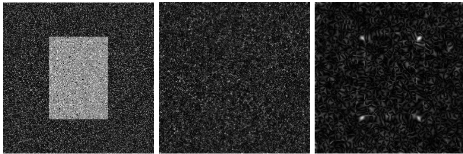
(a) Original image (b) Kitchen-Rosenfeld ( \sigma = 1 ) (c) Kitchen-Rosenfeld ( \sigma = 3 )
