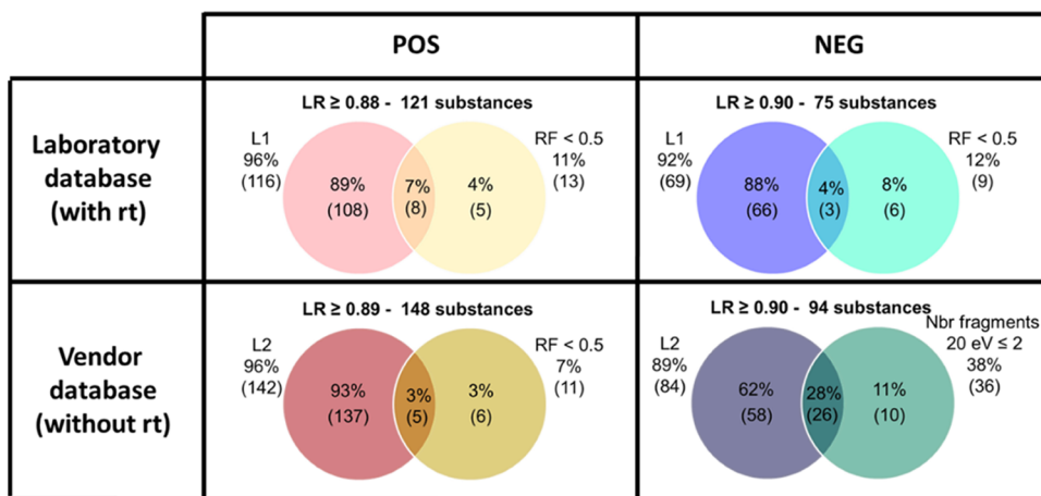
Figure 2. Performances with the highest possible confidence levels obtained depending on the model/databases used and the ionization modes (LR, logistic regression; RF, random forest; rt, retention time; L1/L2, level 1/2; in bracket, number of substances for each category).
