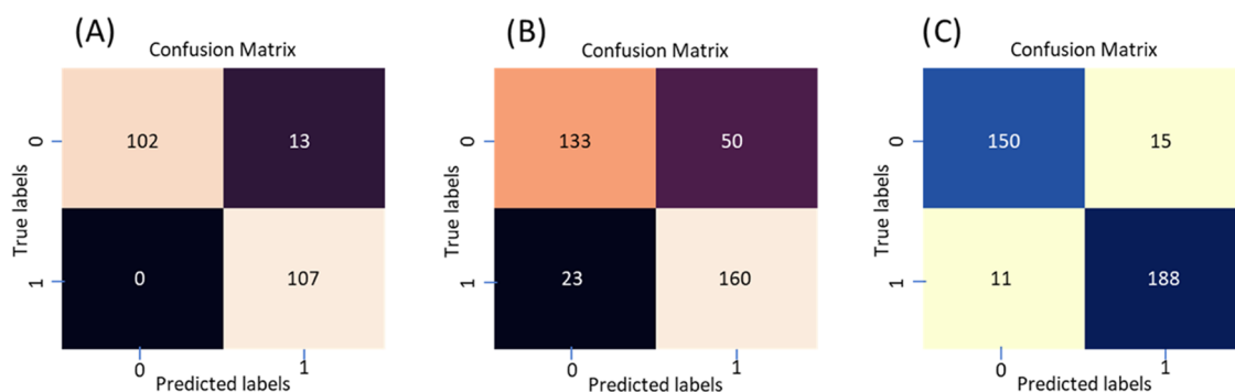
Figure 1. Confusion matrix on the selected model using (A) laboratory database (Study A), (B) vendor database (Study B), and (C) MassBank database (Study C).
