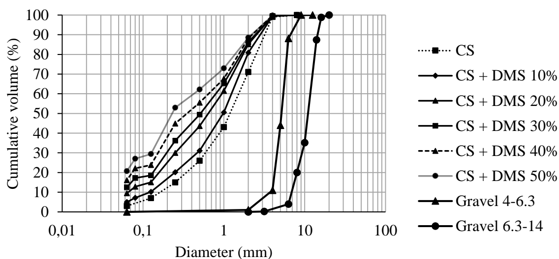
Figure 3. Particle size distributions of sand and gravels used in this study. CS: crushed sand. DMS: Dredged marine sediment.
