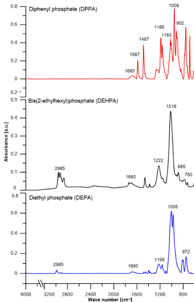
Figure 3. ATR/FT-IR spectra of phosphate samples.
