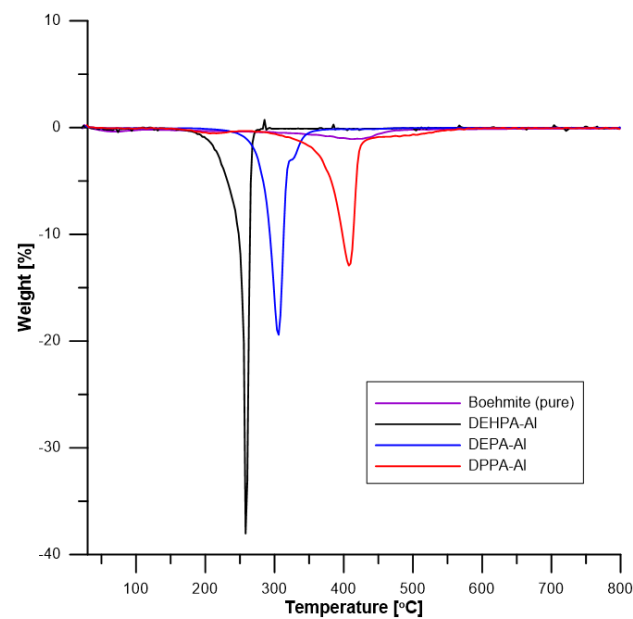
Figure 7. DTG curves of boehmite and hybrids (in helium).
