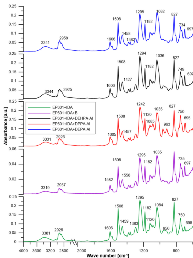
Figure 8. ATR/FT-IR spectra of composites.
