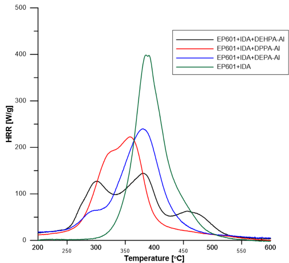
Figure 9. PCFC graphs for obtained composites.
