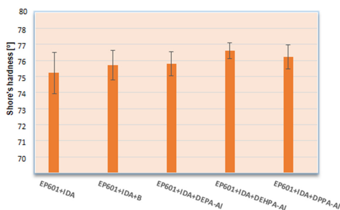
Figure 12. Shore's hardness of composites.
