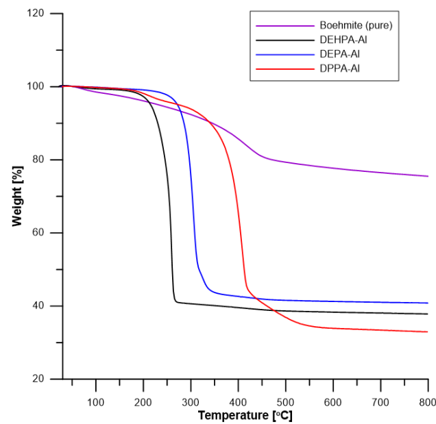
Figure 6. TG curves of boehmite and hybrids (in helium).
