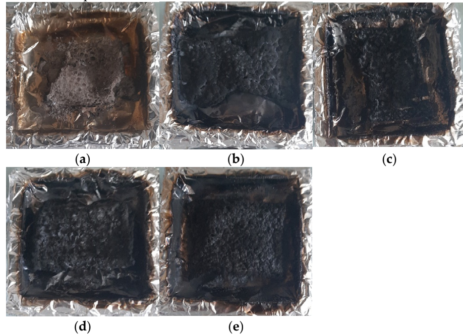
Figure 11. Photos of residue from cone calorimetry tests: (a) EP601 + IDA, (b) EP601 + IDA + B, (c) EP601 + IDA + DEHPA-Al, (d) EP601 + IDA + DPPA-Al, (e) EP601 + IDA + DEPA-Al.
