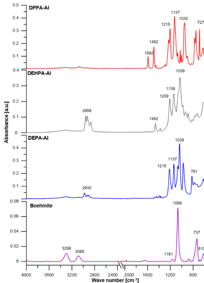
Figure 4. ATR-FT/IR spectra of boehmite and hybrids [cm -1 ].
