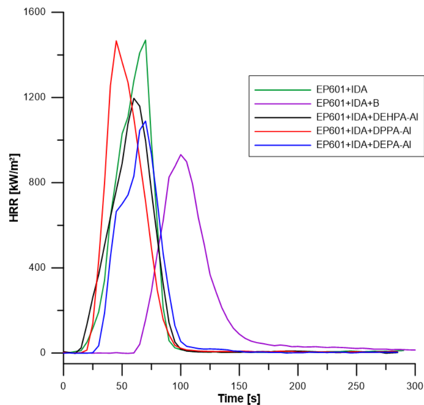
Figure 10. Cone calorimetry graphs for obtained composites.
