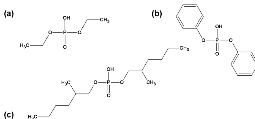
Figure 1. Structure of phosphates: (a) diethyl phosphate (DEPA—20 wt% of phosphorus), (b) diphenyl phosphate (DPPA—12.4 wt% of phosphorus), (c) bis(2-ethylhexyl)phosphate (DEHPA—10.5 wt% of phosphorus).
