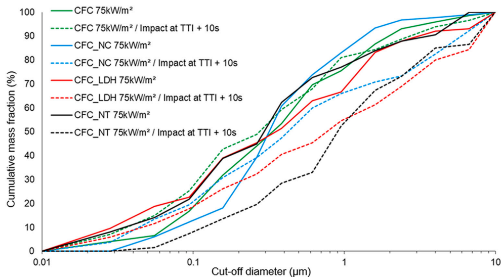
Fig. 5. Cumulative particle-size mass distribution of CFC, CFC_NC, CFC_LDH and CFC_NT samples in both 75 kW/m 2 heat exposure and impact at TTI + 10 s during 75 kW/m 2 heat exposure conditions.
