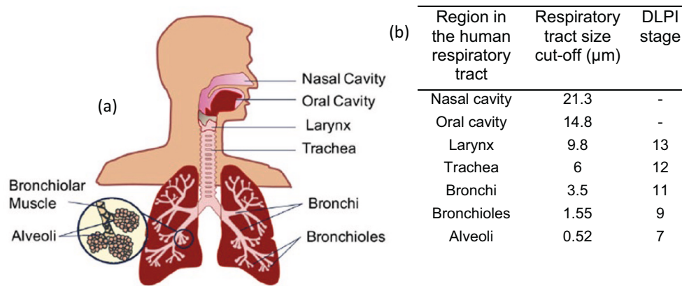
Fig. 4. (a) Respiratory tract and (b) relationship of DLPI stage with soot and particle size cut-off relative to the region of the respiratory tract they are deposited (Rhodes et al., 2011; Lodge Jr, 1987; Rubow et al., 1987). Reproduced with permission from (Rhodes et al., 2011).
