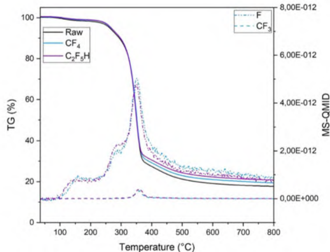
Fig. 9. ATG-MS curves for raw and plasma fluorinated samples.
