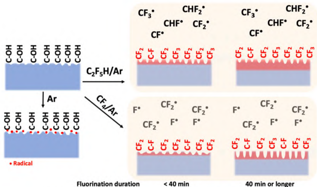
Fig. 7. Schematic view of the fluorination mechanism in \text{C}_2\text{F}_5\text{H}/\text{Ar} and \text{CF}_4/\text{Ar} plasmas.
