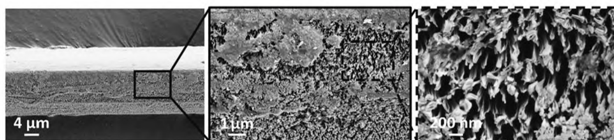
Fig. 5. SEM pictures of etched fibers by \text{CF}_4/\text{Ar} -10 min plasma treatment and zoom on etched area.
