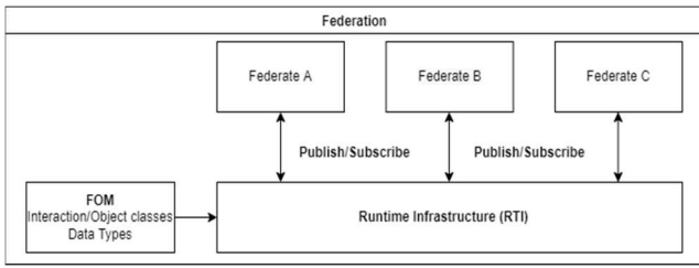
Fig. 1. HLA architecture
