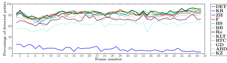
(a) Percentage of matched points per detector along 50 successive images
