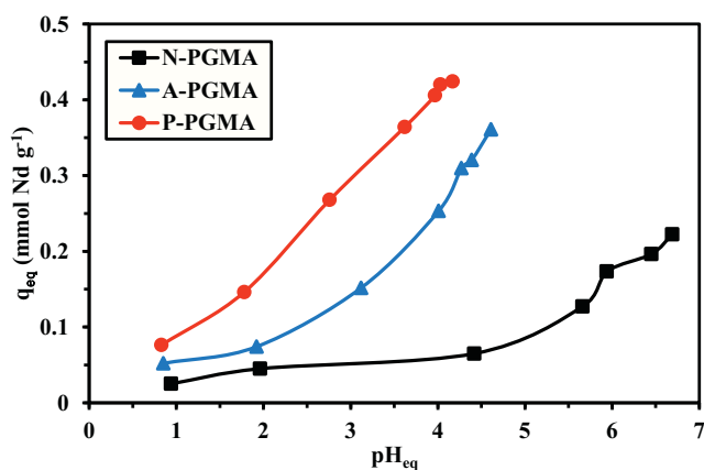
Fig. 2. Effect of pH_{eq} on the sorption of Nd(III) using N-PGMA, A-PGMA, and P-PGMA ( C_0 : 0.347 mmol Nd L^{-1} ; SD: 0.5 g L^{-1} ; Time: 720 min; T: 26 ^{\circ}C ; v: 200 rpm).
