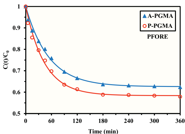
Fig. 3. Uptake kinetics of Nd(III) using A-PGMA and P-PGMA – Using the PFORE for modeling ( \text{pH}_0 : 4.63; SD: 0.5 \text{ g L}^{-1} ; C_0 : 0.744 \text{ mmol Nd L}^{-1} ; T: 26 \text{ }^\circ\text{C} ; v: 200 rpm).
