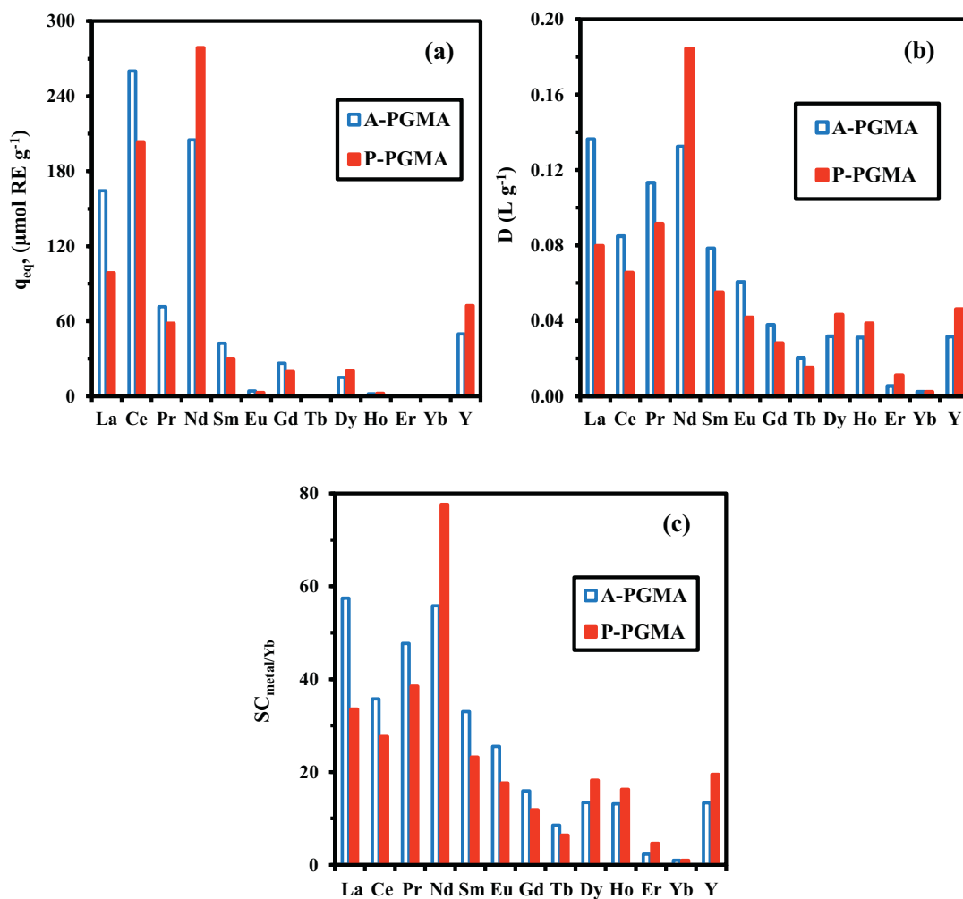
Fig. 6. Sorption tests for the recovery of REEs from pre-treated monazite leachate: (a) sorption capacities, (b) distribution ratio, and (c) SC_{\text{metal/Yb}} ( pH_0 : 4.02; SD: 0.5 g L^{-1} ; time: 120 min; v: 200 rpm; T: 55 \pm 1 °C).
