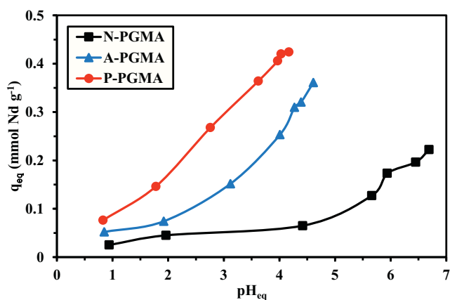
Fig. 2. Effect of pH_{eq} on the sorption of Nd(III) using N-PGMA, A-PGMA, and P-PGMA ( C_0 : 0.347 \text{mmol Nd L}^{-1} ; SD: 0.5 \text{g L}^{-1} ; Time: 720 min; T: 26 ^{\circ}\text{C} ; v: 200 rpm).
