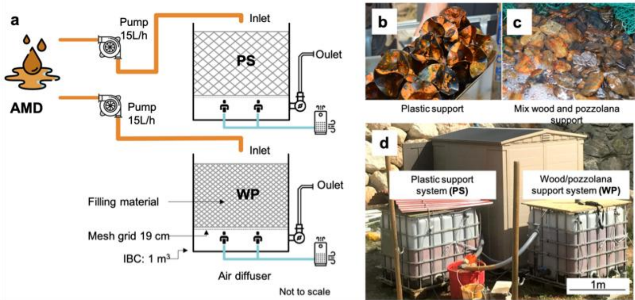
Fig. 1 a) Schematic representations of the biological oxidative devices, one device filled with a plastic support (PS) and the second device filled with pozzolana and wood mixture (WP), b) plastic support, c) wood and pozzolana mixture support and d) in-situ devices.
