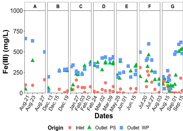
Fig. 4 Variations of the dissolved iron concentration at the inlet and outlet sampling points, for the device with plastic support (PS) and wood/pozzolana support (WP). a) Total dissolved iron (Fe Total), b) Ferrous iron (Fe(II)) and c) ferric iron (Fe(III)). Data collected during seven periods of monitoring: A (Jul.–Aug.19), B (Dec.19), C (Jan.–Feb.20), D (Feb.–Mar.20), E (May–Jun.20), F (Jul.–Aug.20) and G (Aug.–Sep.20). The inlet flow used for the different periods were 15L/h for A, B, C and G while 30L/h for D, E and F represented with black dots in Fig. 4a.
