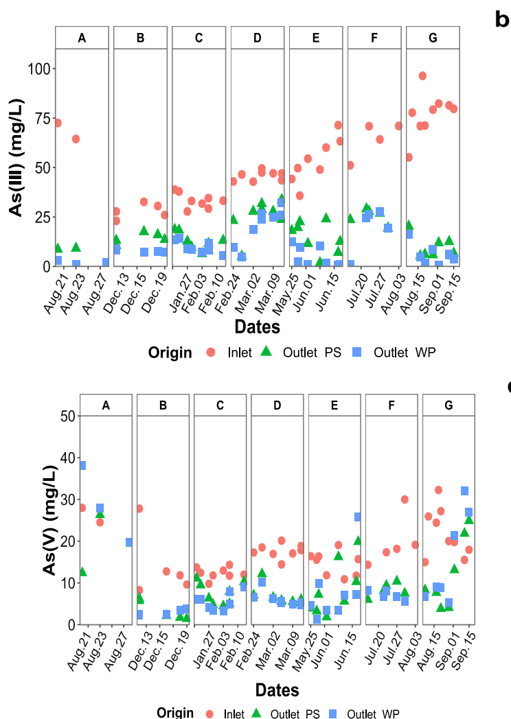
Fig. 5 Variation of the concentration of a) total dissolved (As Total), b) arsenite (As(III)) and c) arsenate (As(V)) at the inlet and outlet sampling points for the device with plastic support (PS) and wood/pozzolana support (WP) during the different periods of operation. The inlet flow used for the different periods were 15L/h for A, B, C and G while 30L/h for D, E and F represented with black dots in Fig. 5a.
