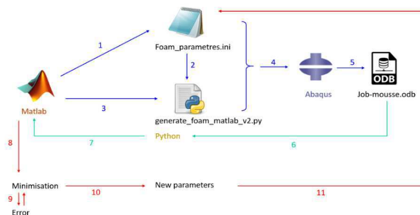
Figure 9: Interface Abaqus-Matlab-Python
