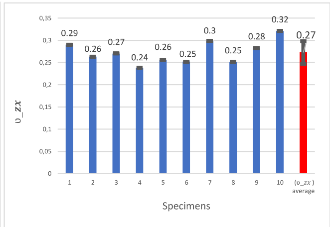
Figure 3: Apparent transverse contraction coefficient \nu_{zx}
