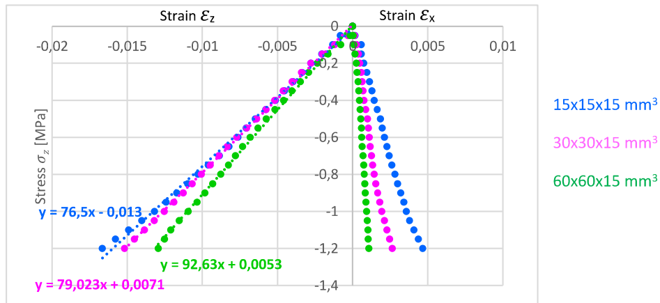
Figure 4: Experimental results PVC80 - Compression tests (3 specimen's dimensions)
