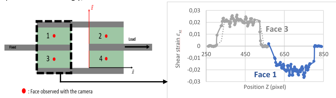
Figure 7: Strain evolution profile - specimen 1
