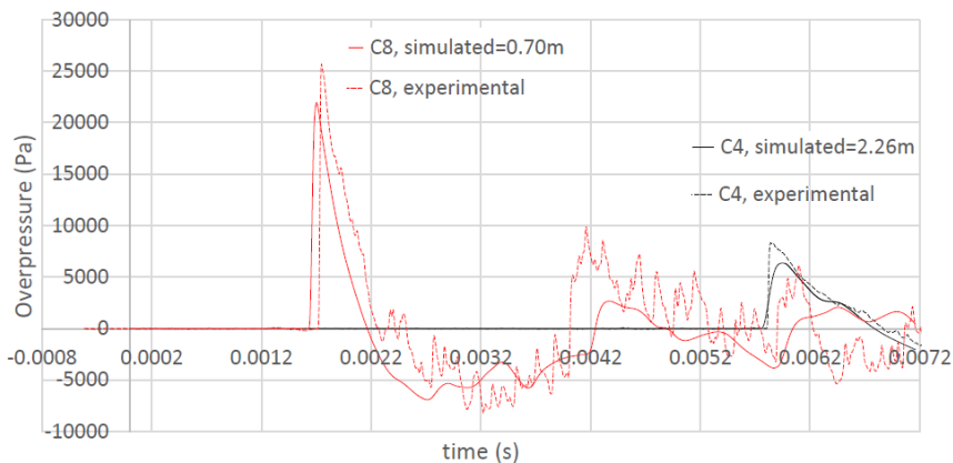
Figure 5: Comparison of experimental results with CFD simulation on the horizontal axis
