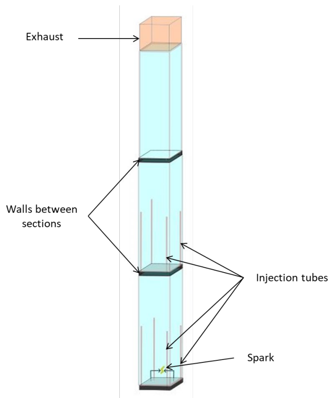
Figure 1: Experimental setup
