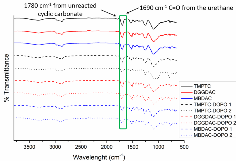
Figure 13: FTIR analyses of the different foams
