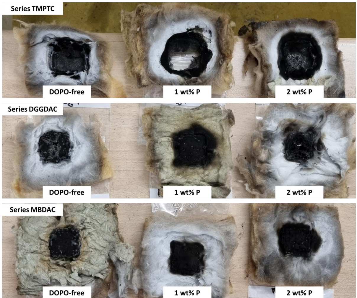
Figure 22: Residues of the foams after cone calorimeter test
