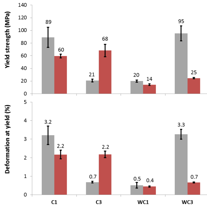
Fig.1 Flexural properties of neat PLA (grey bars) and PLA/flax fiber composite (red bars) obtained by compression molding at the initial state (C1), after reprocessing (C3), after weathering (WC1) and after reprocessing of weathered samples (WC3)
