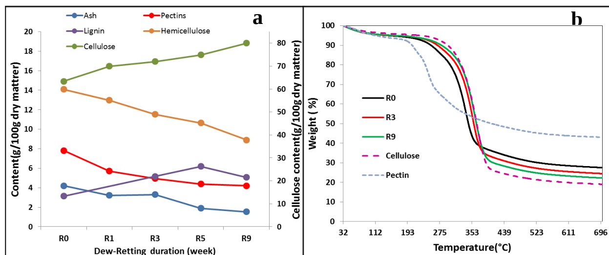
Figure 1 : Evolution of the biochemical content of fibers at the beginning of flowering A) Hemp fibers content variation using solvent extraction. B) Mass loss of hemp fibers content during dew-retting by thermogravimetry.
