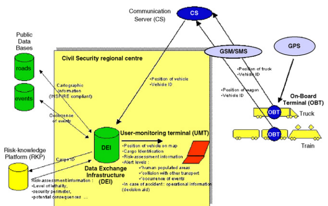
Fig. 1. MITRA prototype system architecture.
