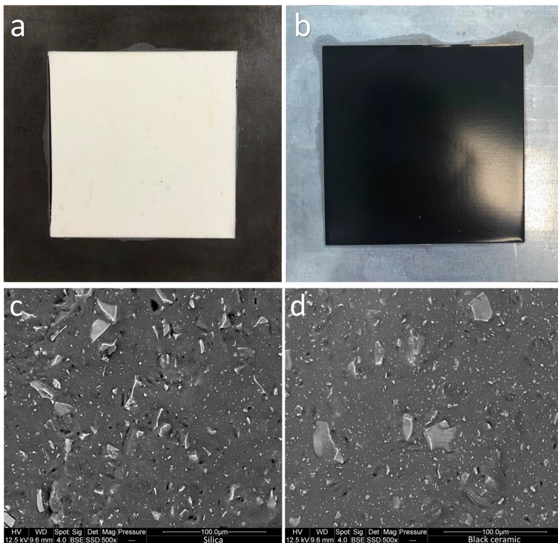
Fig. 4. (a, b) Photographs of the elastomers containing 30 wt% of silica powder (a) and black ceramic powder (b) after peroxide crosslinking; (c, d) Corresponding SEM micrographs of elastomers filled with silica powder (c) and black ceramic powder (d). Note that the black spots observed on the SEM micrographs are ascribed to an incomplete metallization (see also Figure S3).
