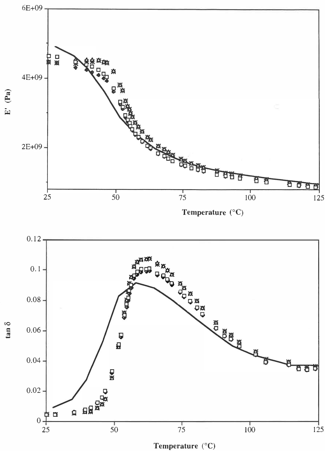
Figure 7. Choice of the prediction method of the matrix Poisson's ratio: Christensen's model (Kolsky ( \square ), Theocaris ( \triangle )) and Maurer's model ( V_i = 0.01\% /Kolsky ( \blacklozenge ), Theocaris ( * )) compared to experimental data (—) obtained for 40 wt% of aminosilane treated glass beads.
