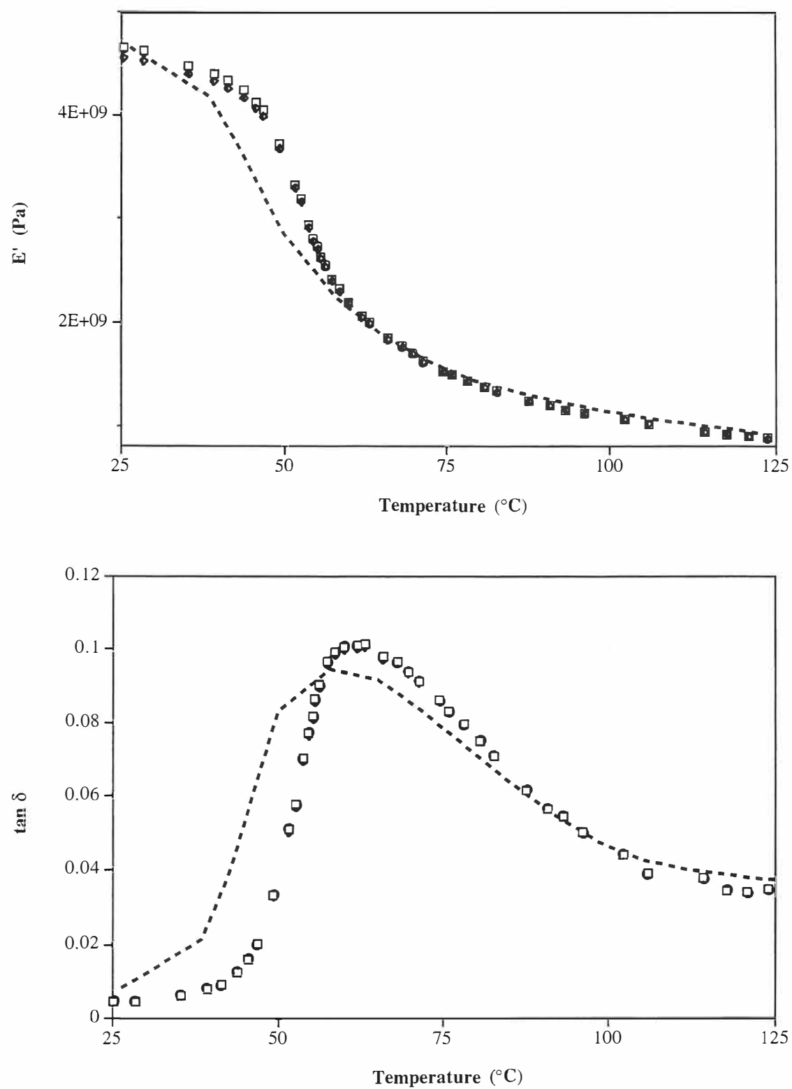
Figure 8. Theoretical curves based on the self-consistent models of ( \blacklozenge, \circ ) Maurer and ( \square ) Christensen. Comparison with a poly(butylene terephthalate) reinforced by (- - -) 40 wt% of vinylsilane treated glass beads. (Volume fraction of interphase ( \blacklozenge ) 0.01% and ( \circ ) 0.05%.)
