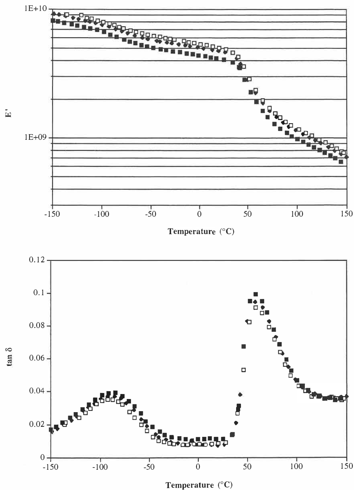
Figure 2. Curves of E' and \tan \delta versus temperature at 5 Hz for a poly(butylene terephthalate) reinforced by 40 wt% of (■) untreated glass beads or coated by (◆) a vinylsilane and (□) an aminosilane coupling agent.
