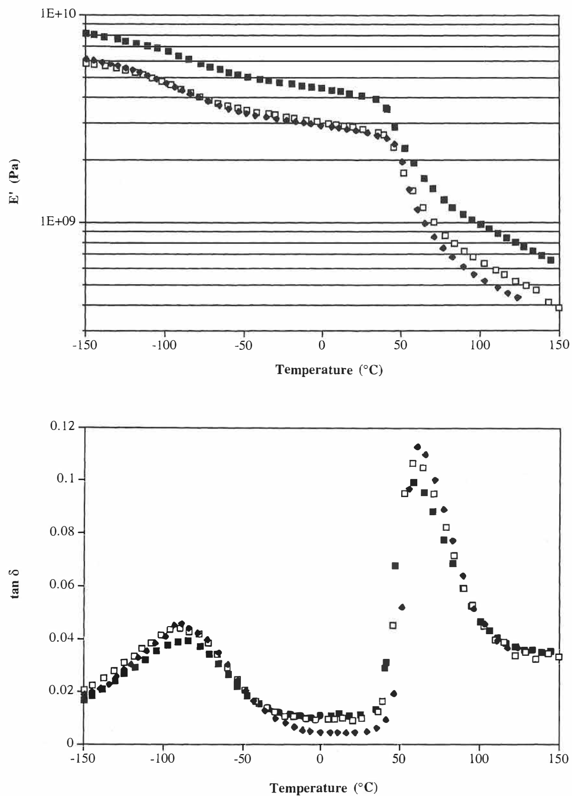
Figure 1. Curves of E' and \tan \delta versus temperature at 5 Hz for (◆) a pure poly(butylene terephthalate) and reinforced by (□) 15 wt% and (■) 40 wt% of untreated glass beads.
