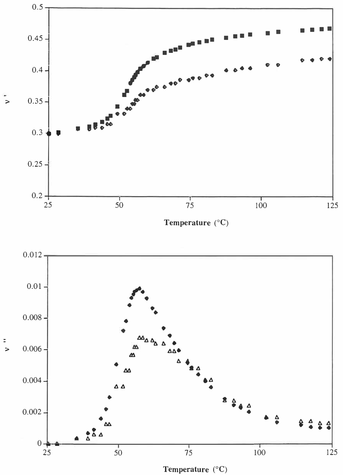
Figure 6. Theoretical curves of Poisson's ratio versus temperature for a poly(butylene terephthalate) matrix: Kolsky's (■) \nu' , (◆) \nu'' and Theocaris' (◊) \nu' , (△) \nu'' approaches.
