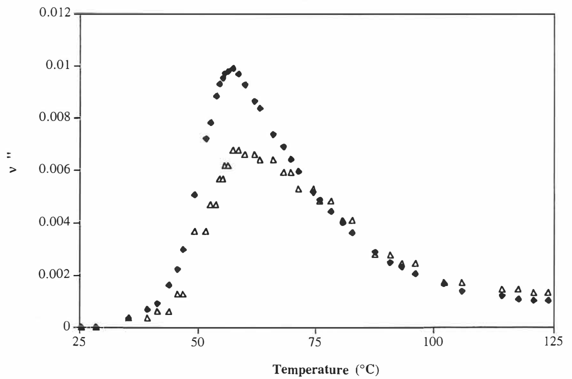
Figure 6. Theoretical curves of Poisson's ratio versus temperature for a poly(butylene terephthalate) matrix: Kolsky's (■) \nu' , (◆) \nu'' and Theocaris' (◄) \nu' , (△) \nu'' approaches.
