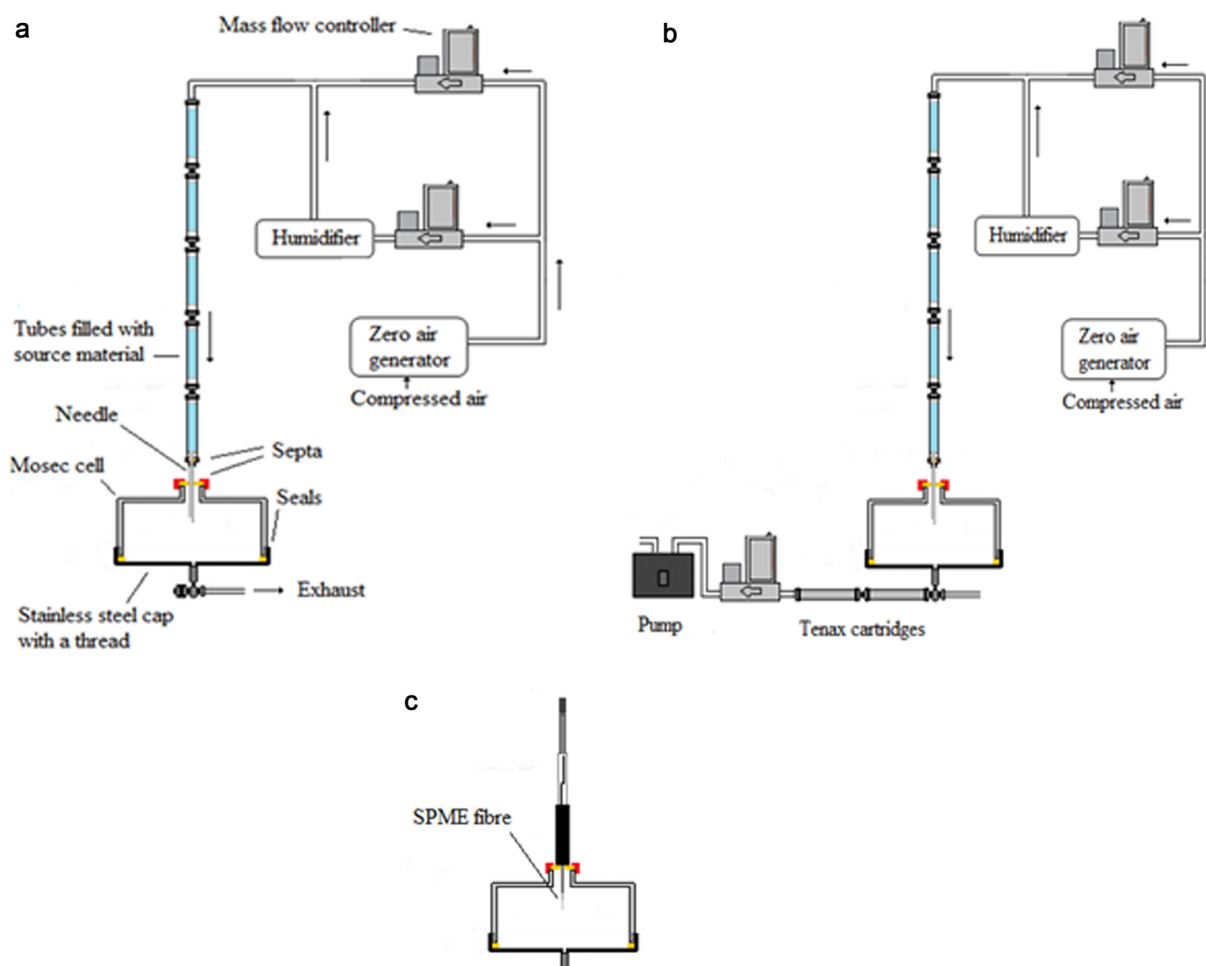
Fig. 2. Fig. 2-a-A calibration atmosphere generation system (without device for Tenax sampling) [26]; Fig. 2-b-Calibration atmosphere generation system (with device for Tenax sampling) [26]; Fig. 2-c -SPME sampling in isolated emission cell [26].
