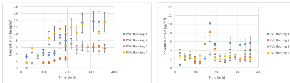
Fig. 6. A Gas-phase concentration of DBTP versus time after that the MOSEC cell is placed on the PVC floorings; Fig. 6-b–Gas-phase concentration of DiBP versus time after that the MOSEC cell is placed on the PVC floorings.
