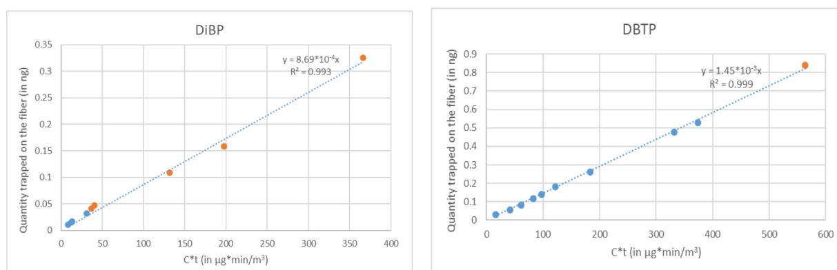
Fig. 5. Calibration curves for DiBP and DBTP. Extracted mass by SPME versus the product of sampling time ( t ) and gas-phase concentration ( C ) by combining the data of two calibration series (blue points are associated with test n^{\circ}1 and orange with n^{\circ}2 ).
