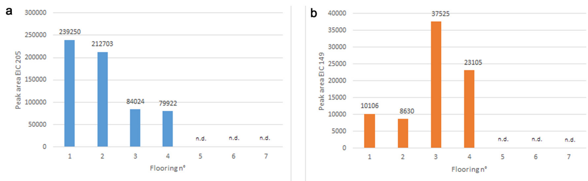
Fig. 3. Fig. 3-a-A peak areas obtained by HS-SPME-GC-MS/FID for DBTP; Fig. 3-b-Peak areas obtained by HS-SPME-GC-MS/FID for DiBP.
