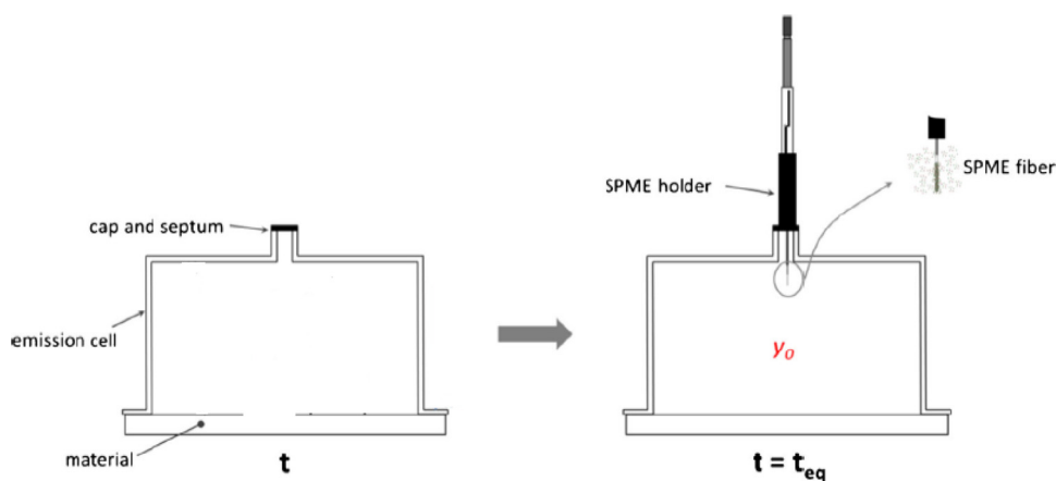
Fig. 1. illustration of the MOSEC cell [26].
