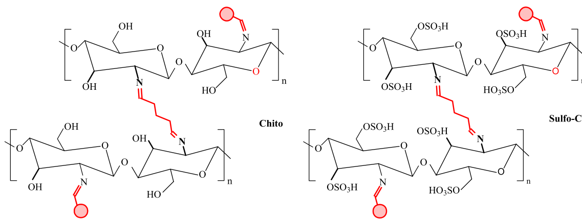
Scheme 1. Suggested structures for Chito and Sulfo-C sorbents.
