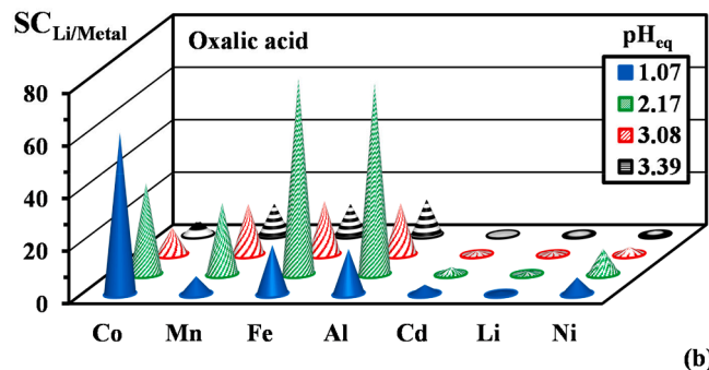
Fig. 8. Effect of pH on the selectivity coefficient ( SC_{Li/metal} ) for metal sorption from battery leachate using Sulfo-C sorbent – without (a) and with oxalic acid (1%, w/w) (b) (SD: 1\ g\ L^{-1} ; Time: 10 h; v: 210 rpm).
