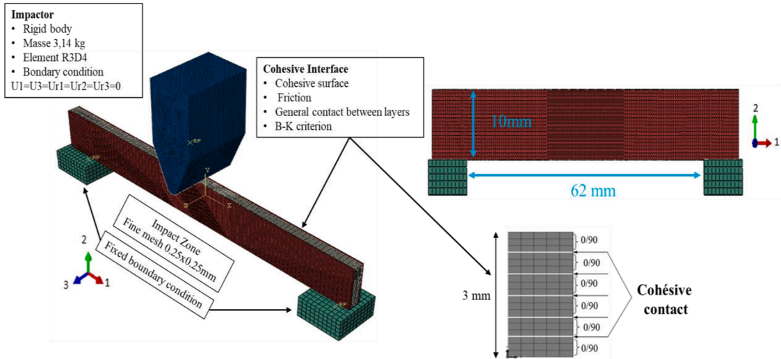
Fig. 14. Finite element model of a sample subjected to impact.
