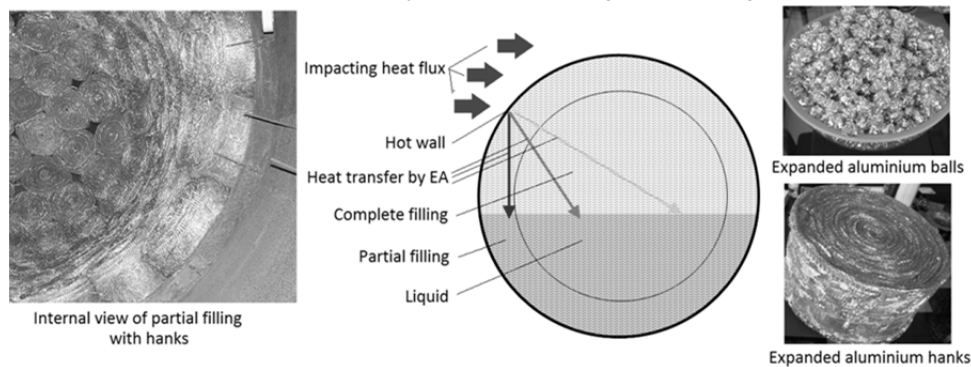
Figure 1: Expanded aluminium configurations and assembly in a reservoir
