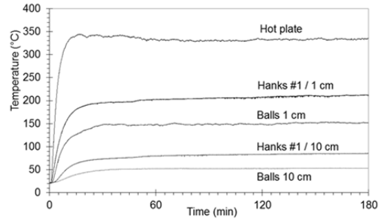
Figure 5: Hot plate and EA temperatures
