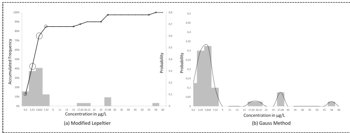
476 Figure 4: Distribution of concentrations for one type of geological formation according to Lepeltier (left) and 477 Gauss (right) methods. Example for arsenic on metamorphic basement. The cases of arsenic and antimony on 478 the different types of geological formations are represented in Supplementary Information, (Figures SI-2 and SI- 479 3).
